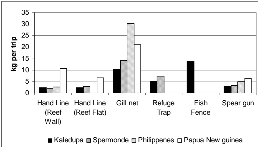
Figure 1. Catch Per unit effort in kg per trip, for Kaledupa (2003), West Spermonde Archipelago, Malalison Island (Philippines) and Papua New Guinea.
